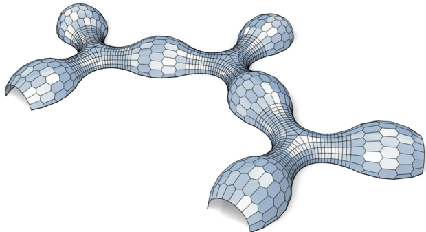
Figure 19: This design with convex faces is composed from pieces of discrete cmc surfaces obtained in different ways. The junction piece (quad mesh) was originally computed as a tri-noid (cf. [Grosse-Brauckmann and Polthier 1997; Schmitt 2004]) by the applet at [Schmitt 2003]. After combined optimization of mesh and Gauss image in order to achieve planarity of faces and H_F = \text{const.} , we arrive at a planar quad mesh which has H_F \in [0.966, 1.048] . The bulging pieces are hexagonal EO meshes whose mean curvature with respect to a previously chosen Koebe polyhedron as Gauss image is exactly constant.
