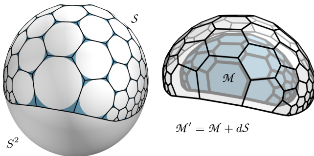
Figure 8: A mesh \mathcal{M} with an edge offset mesh \mathcal{M}' at distance d has a parallel mesh \mathcal{S} = (\mathcal{M}' - \mathcal{M})/d whose edges are tangent to the unit sphere S^2 . The faces of \mathcal{S} intersect S^2 in a circle packing, cf. Section 3.2.
